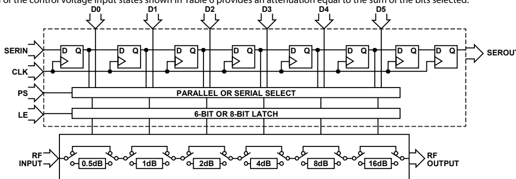
Figure 32. Simplified Circuit Diagram
